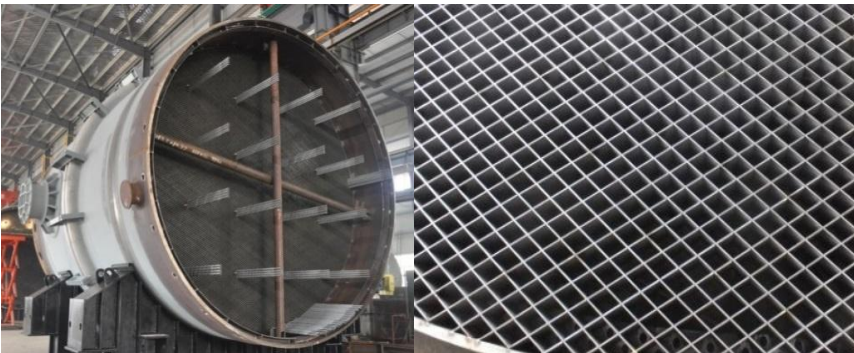
Grating Baffle HE – Coupling Reactor DN6000, 17,793 tubes, 497tons, SS
