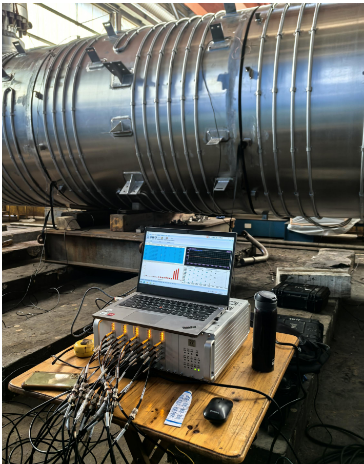
Acoustic Emission Testing (AET)
