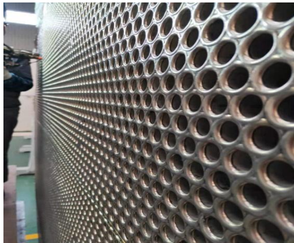
Tube-to-Tubesheet
