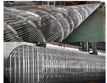
Rod Baffle Heat Exchanger
