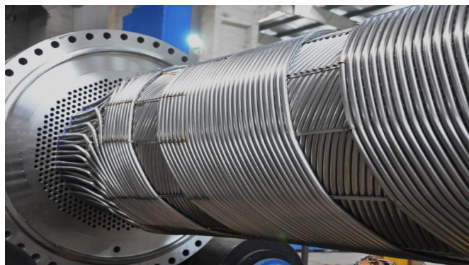
LNG Plant Liquefaction Condenser DN2600*11,671mm F = 2,640m 2 ; 95 tons S30408
