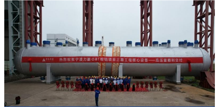
HPAL – AutoClave DN5600*8/134*37000, 1022 ton (Titanium Clad)
