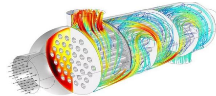
UOP Process PDH Project - High Flux Tube Heat Exchanger CS, Copper Alloy Material (Thailand, Canada)
